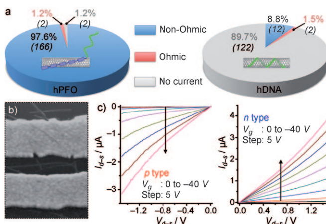
Figure 5. FET device fabrication with hPFO. a) Comparison of fabrication efficiencies, 99% and 10% bridging in total, for hPFO (left) and hDNA (right) devices, respectively. Numbers in parentheses denote the number of devices that exhibit the corresponding electrical behavior. b) SEM image of a sample bridging region from a hPFO device. c) FET characteristics for a representative hPFO device showing ambipolarity. Output curves in p- and n-type ranges (left and right, respectively). See Figure S26 for the transfer curves of the same device.
